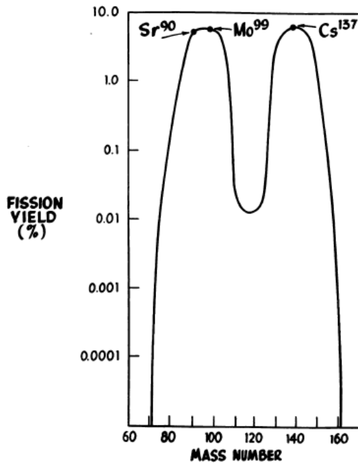
FIG. 3 FISSION PRODUCTS
